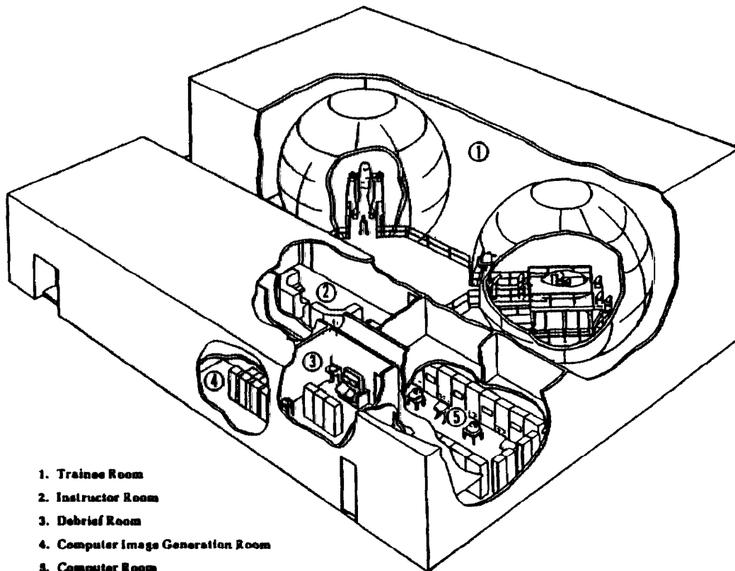
Layout of Weapons Tactics Trainer. Device 2E7
