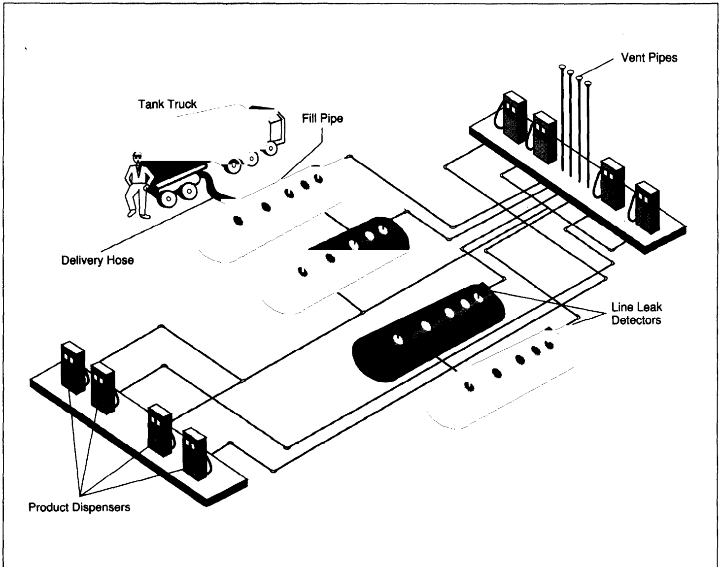
Figure 1.1: A Typical Tank Facility
