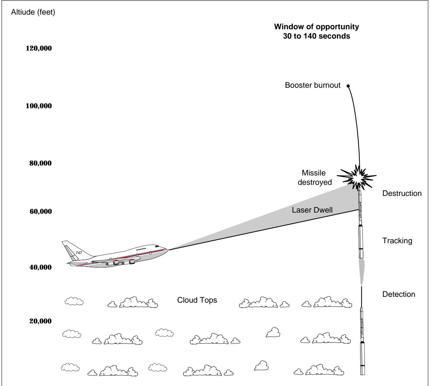
Figure 1: ABL Missile Engagement
