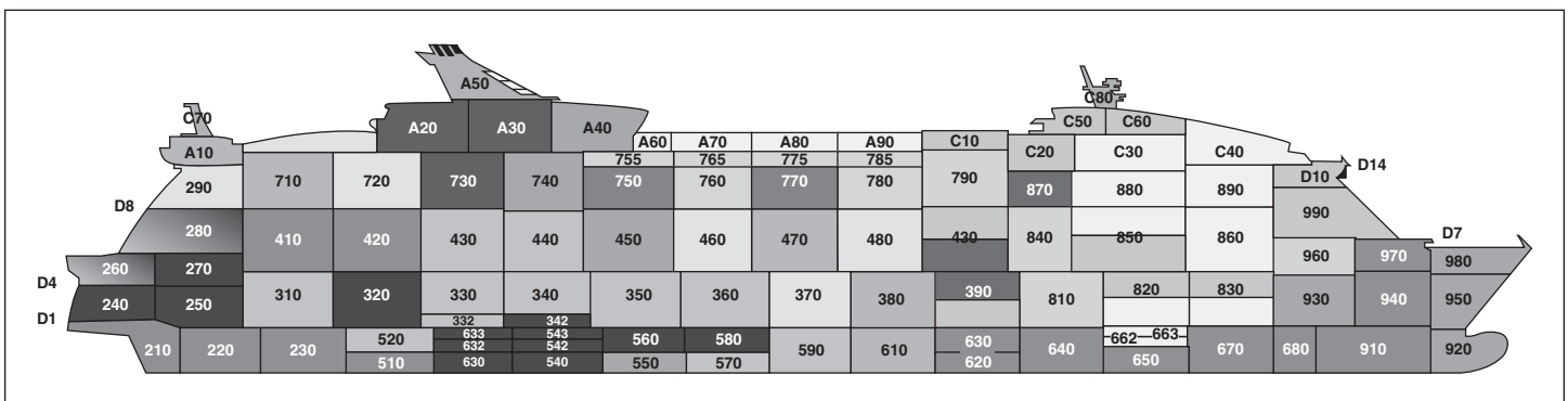
Figure 10: Block Definition Plan for a Cruise Ship
