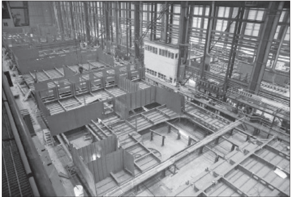
Figure 2: Cruise Ship Block Fabrication
