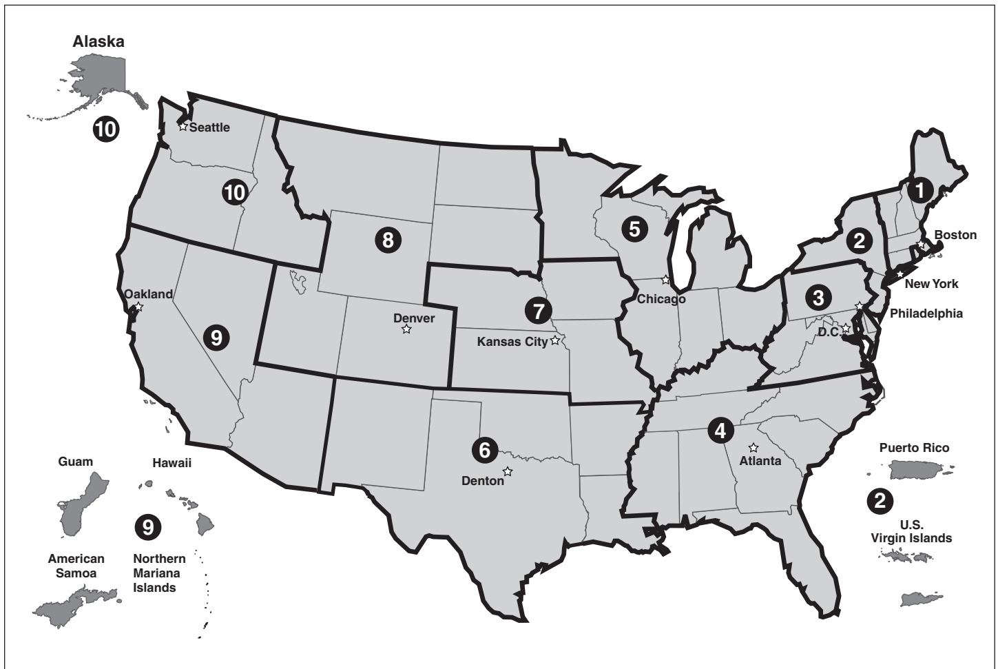
Figure 5: FEMA Regions
