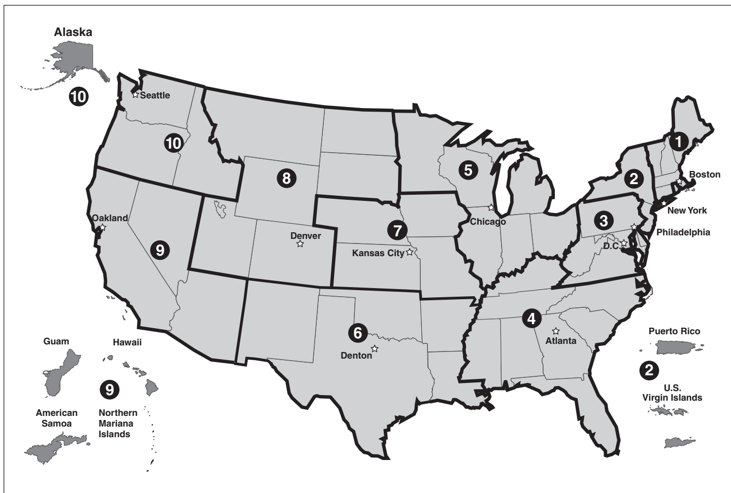
Figure 2: FEMA Regions
