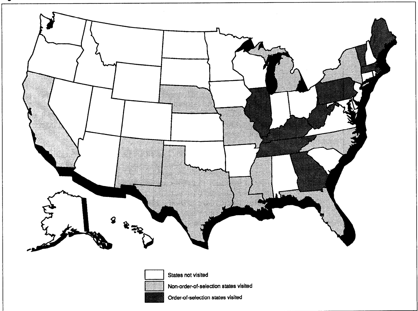
Figure 1.3: States Visited
