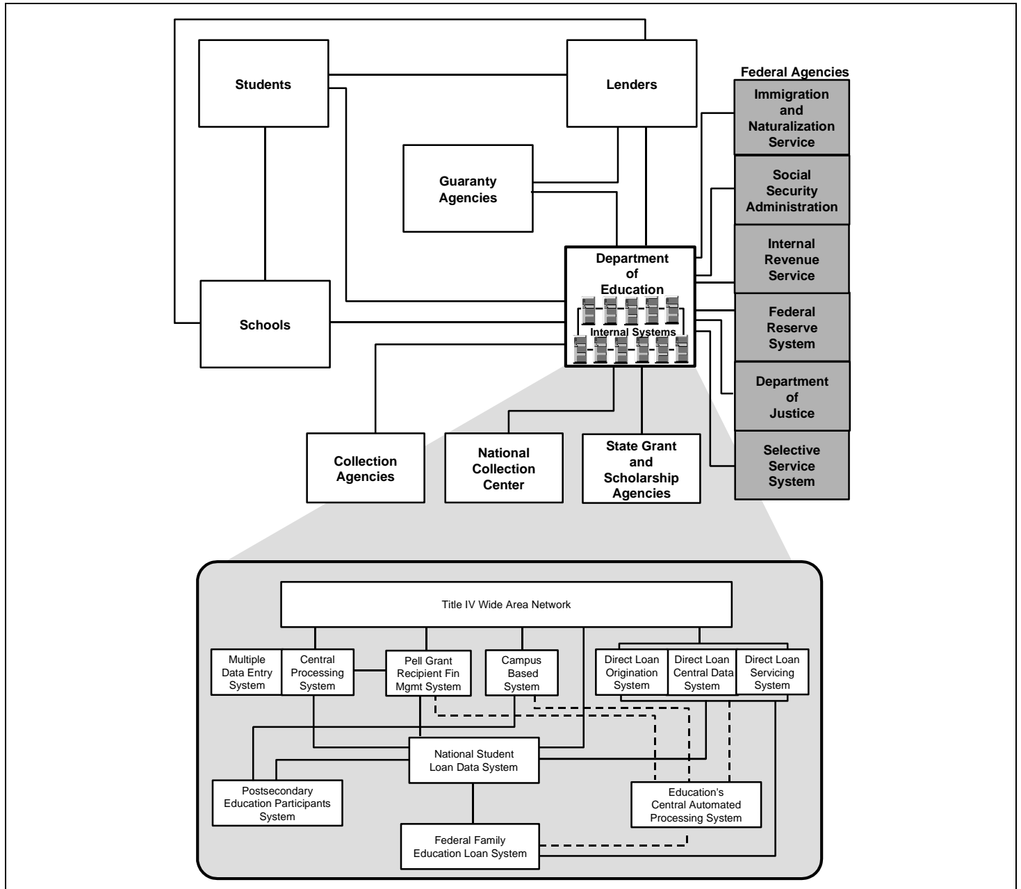
Figure 1: Education's Student Financial Aid Data Exchange Environment
