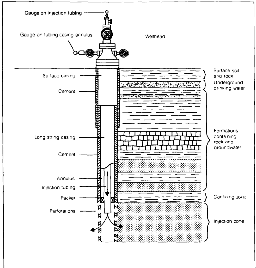
Figure 1.1: Typical Hazardous Waste Disposal Well
