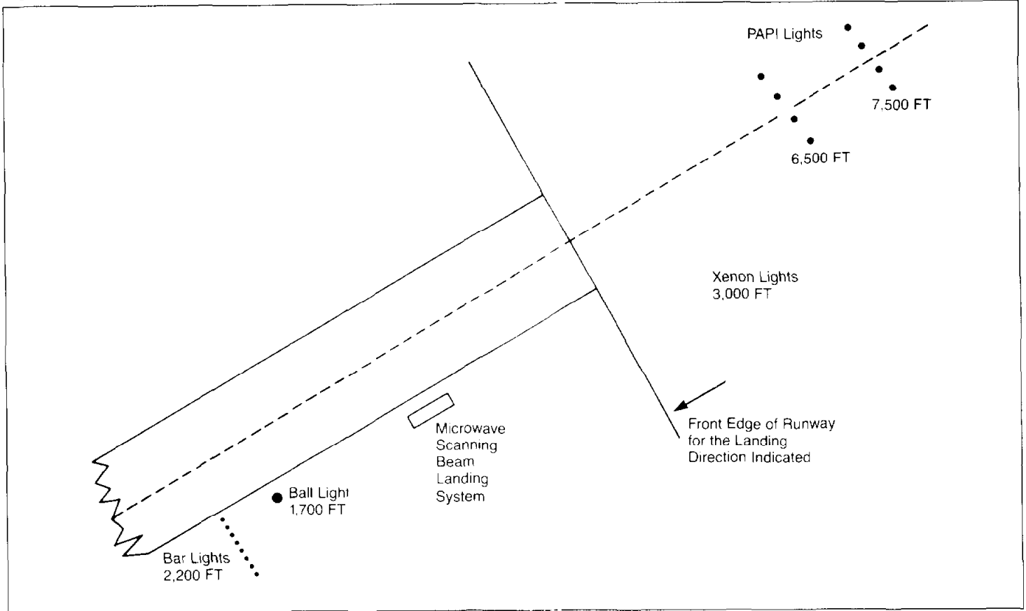
Figure II.7: Positioning of Selected TAL Site Landing Aids
