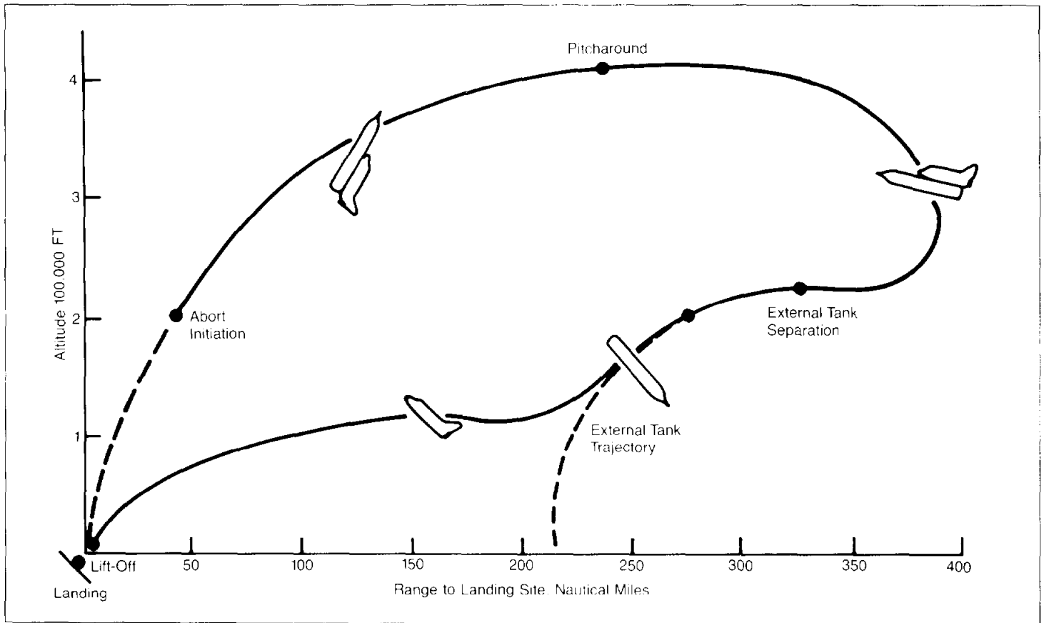
Figure I.1: Return to Launch Site Abort Mode
