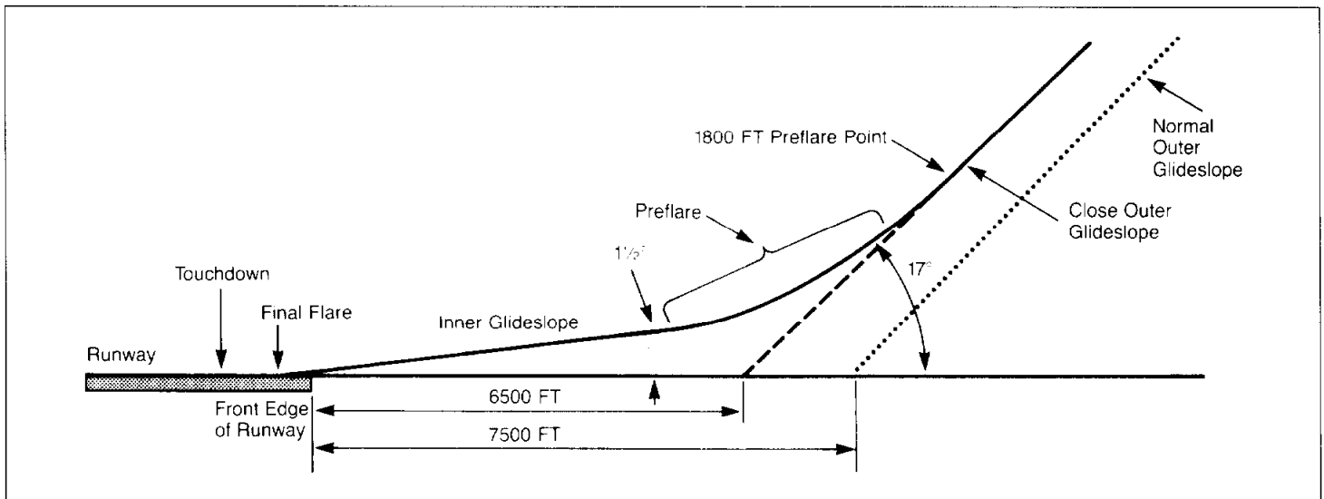
Figure II.5: Shuttle Approach and Landing Geometry
